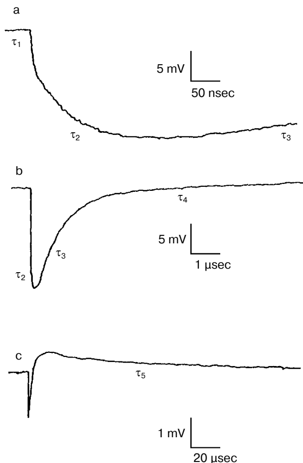
Fig. 12. Electric response signals from purple membrane oriented and immobilized in gel: a–c) signals with different amplitude and time scales ((a) tens of nanoseconds, (b) microseconds, (c) tens of microseconds). Distilled water suspension, temperature 22°C.
