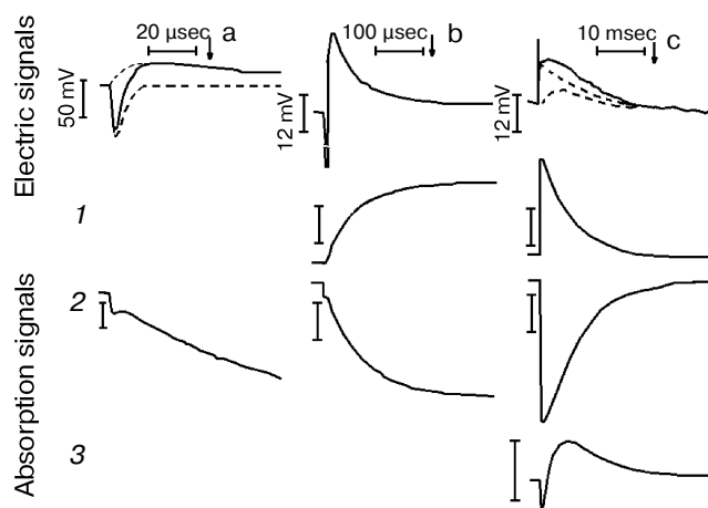
Fig. 1. Comparison of the electric and light absorption signals at different wavelengths: 408 (1), 522 (2), and 635 nm (3). a-c) Signals measured with different time resolution ((a) tens of microseconds, (b) hundreds of microseconds, (c) tens of milliseconds). Dashed lines in columns (a) and (c) denote the decomposition of the electric signals. The size of bars in absorption signals means a 10% change in absorption. Purple membrane in H 2 O solution, orienting field 8.5 V/cm, temperature 20°C.
